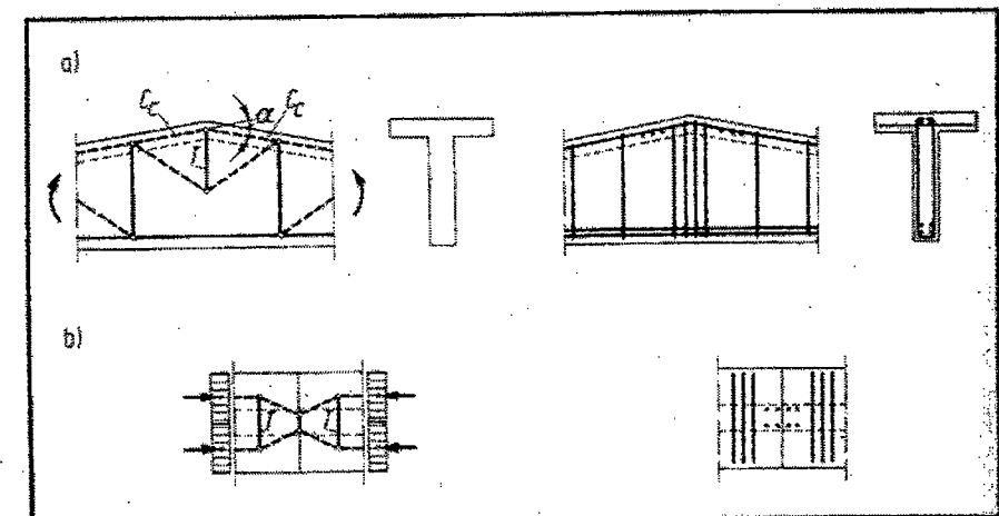
Fig. 47. Girder with berr top flange.
