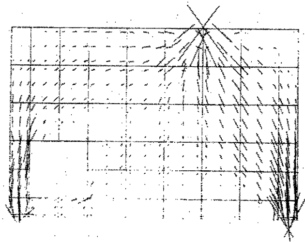
b) elastic stresses
