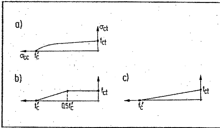
Fig. 26. The biaxial compressive-tensile strength of concrete and two simplified assumptions for analytical application.
