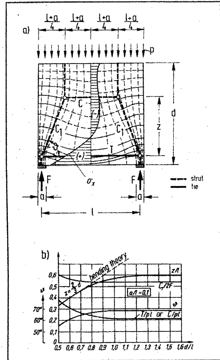
Fig. 9. A typical D-region: (a) elastic stress trajectories, elastic stresses and strut-and-tie-model; (b) diagram of internal forces, internal lever arm z and strut angle \delta .
