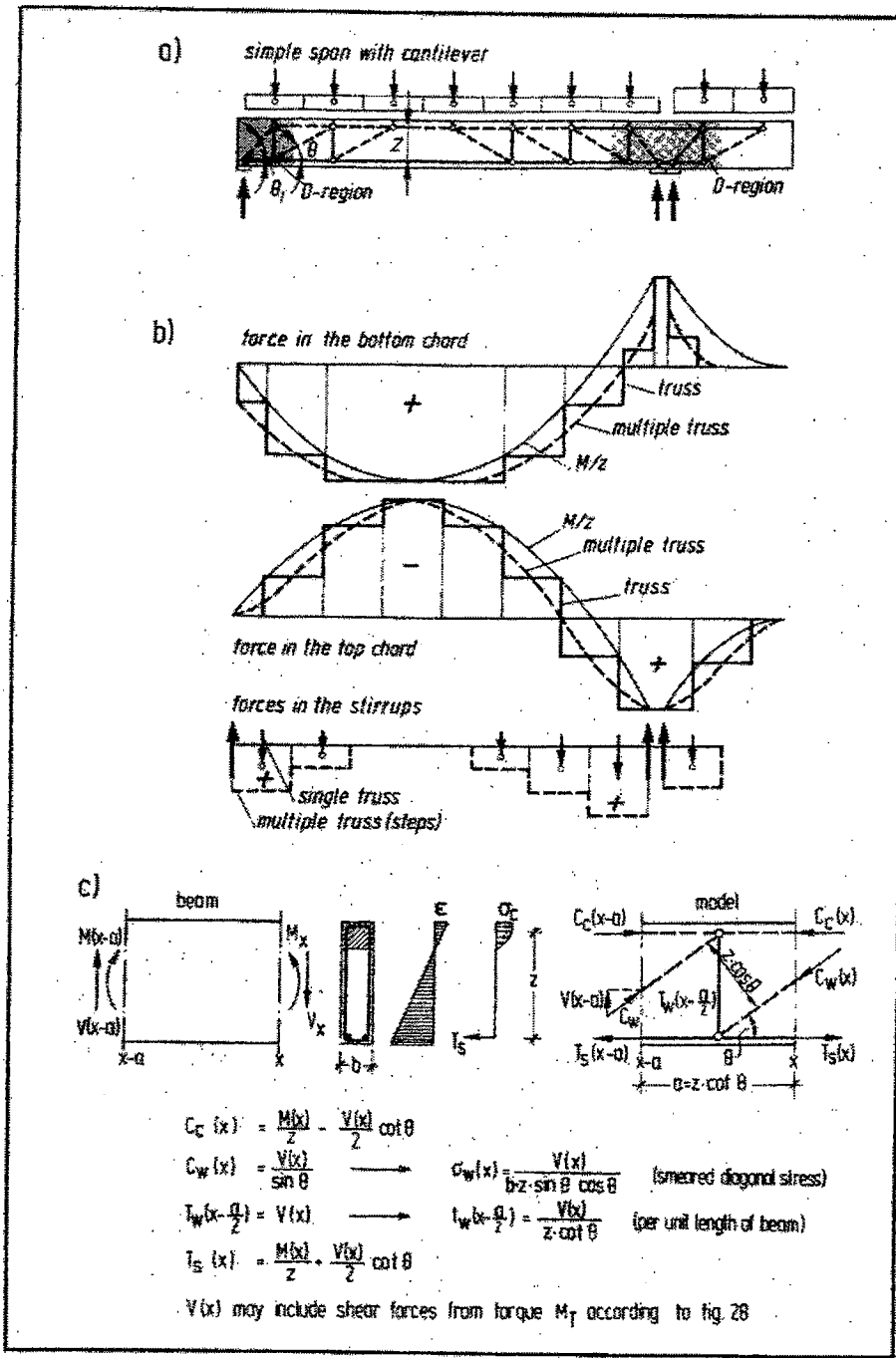
Fig. 8. Truss model of a beam with cantilever: (a) model; (b) distribution of inner forces; (c) magnitude of inner forces derived from equilibrium of a beam element.
