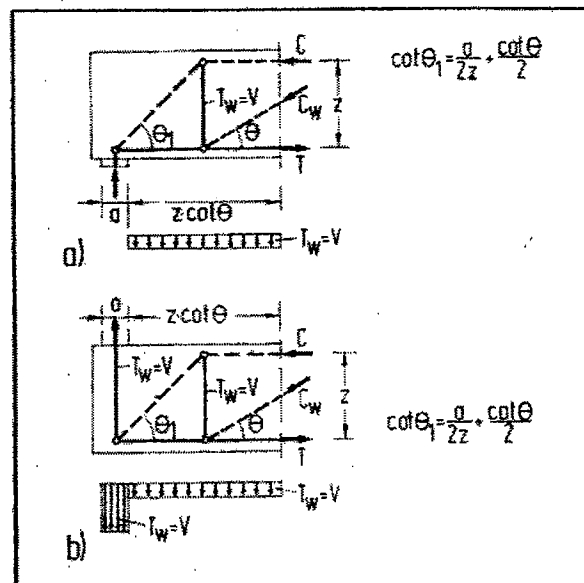
Fig. 39. Detailed geometry of D_2 -region from Fig. 38: (a) direct support; (b) indirect support.
