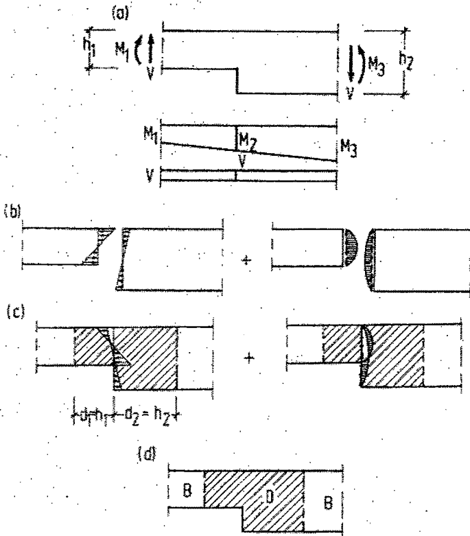
Fig. 3.3. Beam with a recess.
