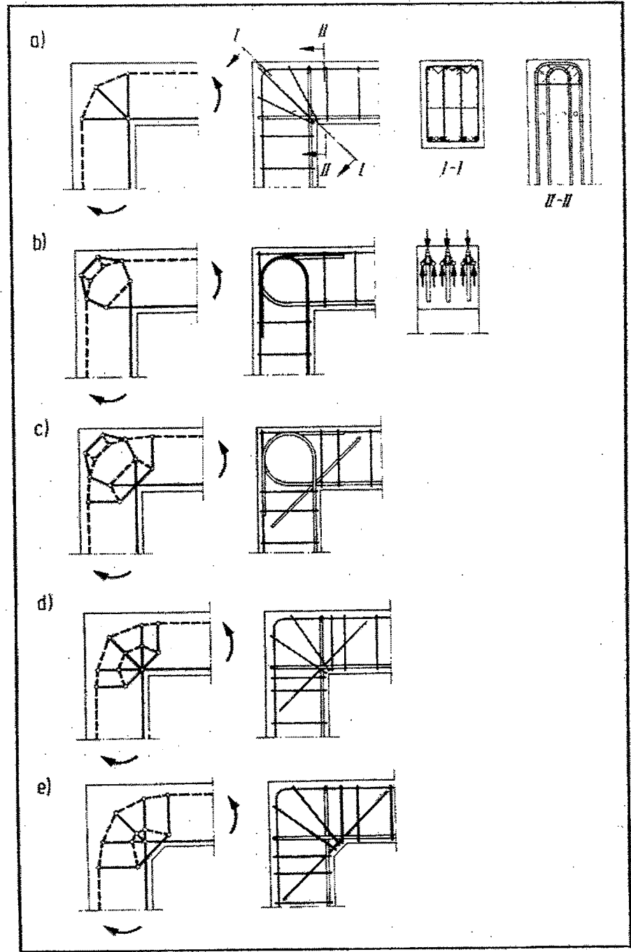
Fig. 49. Different strut-and-tie-models and the corresponding reinforcement for a frame corner with positive moment.
