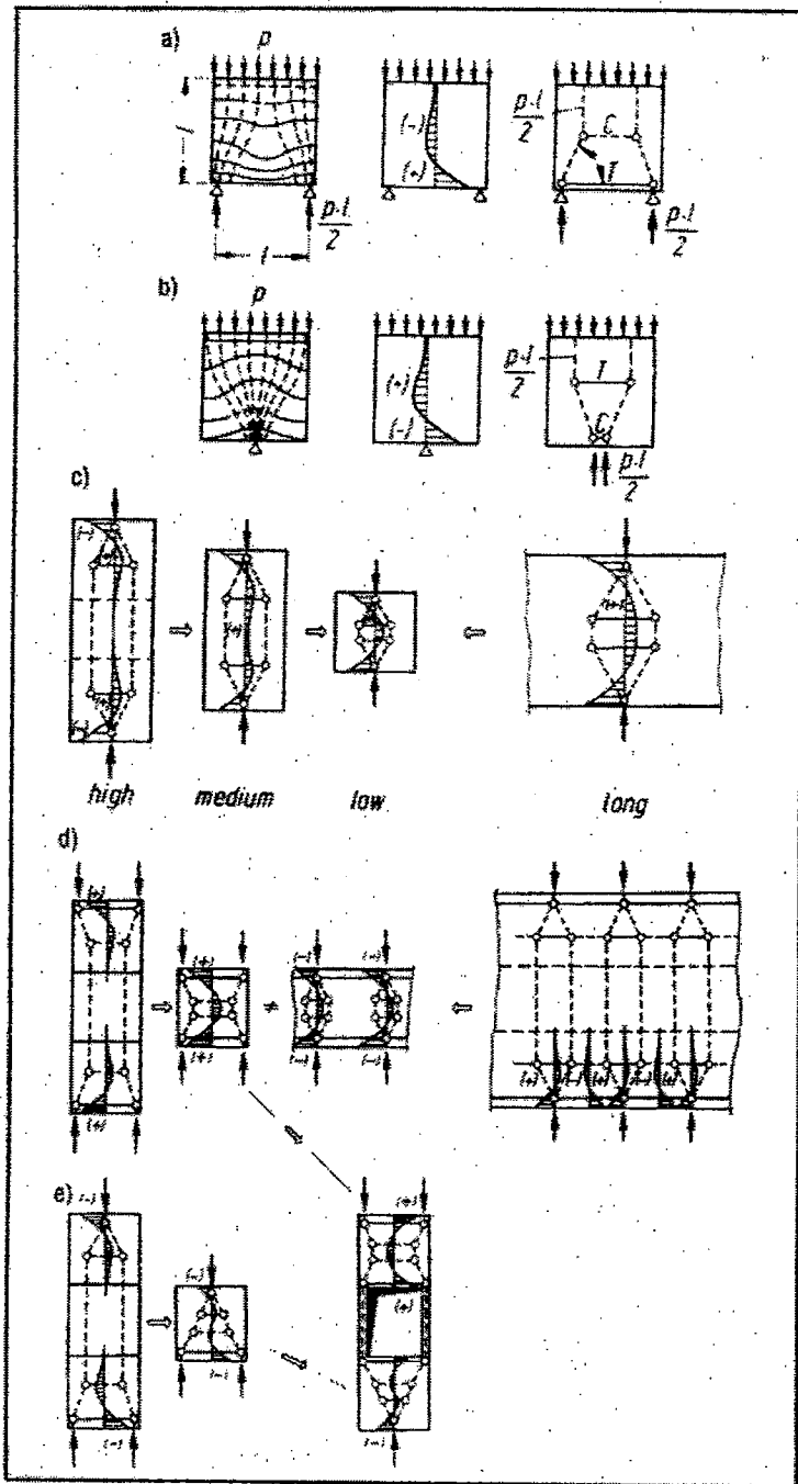
Fig. 15. The two most frequent and most useful strut-and-tie models: (a) through (b), and some of their variations (c) through (e).
