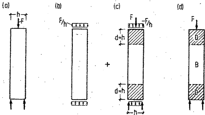
Fig. 3.1. Column with point loads.
