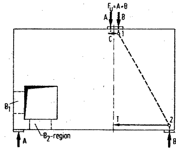
c) load path, right side
