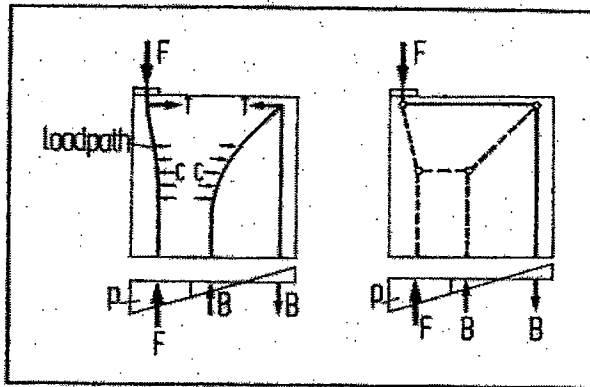
Fig. 11. Load paths (including a "U-turn") and strut-and-tie-model.
