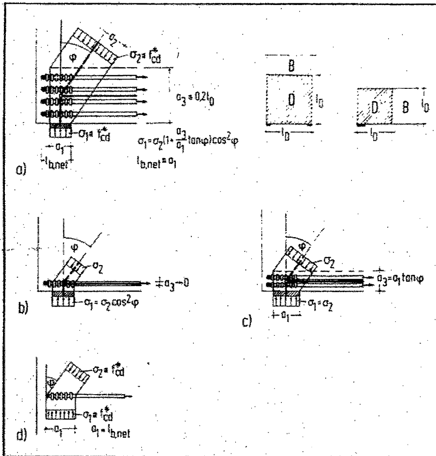
Fig. 22. A proposal for the dimensioning of typical singular CCT-nodes with different reinforcement layouts: (a) multilayered tie ( a_2 relatively large, \sigma_2 < \sigma_1 ); (b) single layer tie ( a_2 small, \sigma_2 > \sigma_1 ); (c) special case in between ( \sigma_2 = \sigma_1 ); (d) same type as (b) with pressure from a compression field.
