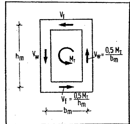
Fig. 28. Shear forces as a result of torsion.
