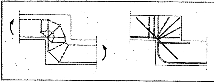
Fig. 48. The stepped beam.
