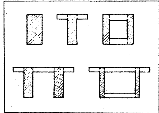
Fig. 27. Various cross sections of beams and their webs.
