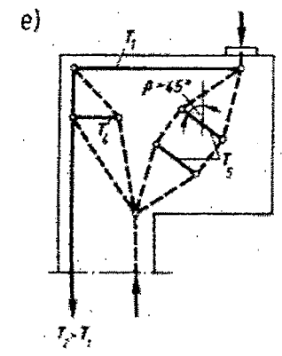
Fig. 40. Different support conditions lead to different strut-and-tie-models and different reinforcement arrangements of corbels.
