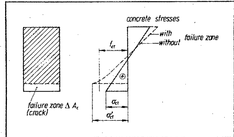
Fig. 25. Progressive failure of a beam because of a local failure zone, which increases maximum tensile stresses \sigma_{ct} to \sigma_{ct} > l_{ct} .
