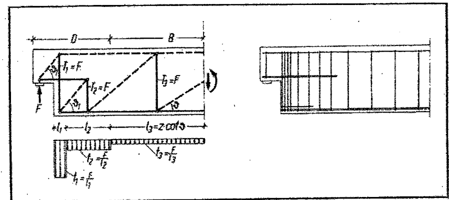
Fig. 46. Beam with dapped end.
