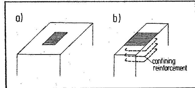
Fig. 21. Confinement (a) by the surrounding concrete; (b) by reinforcement increases the design compression strength f_{cd}^* .
