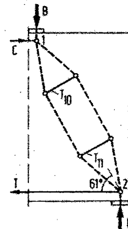
d) complete model, right side
