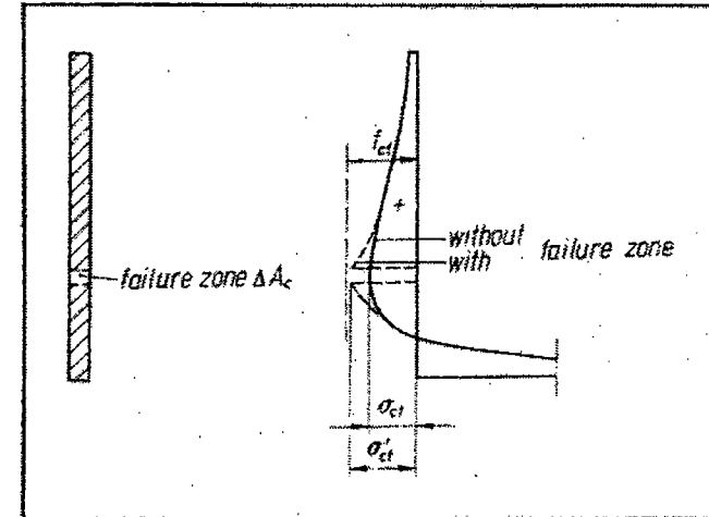
Fig. 24. Assumption of a failure zone for the check of the tensile strength of a concrete tension tie T_s .
