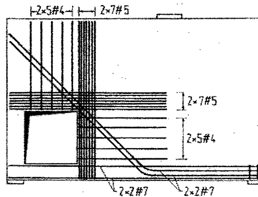
i) reinforcement
