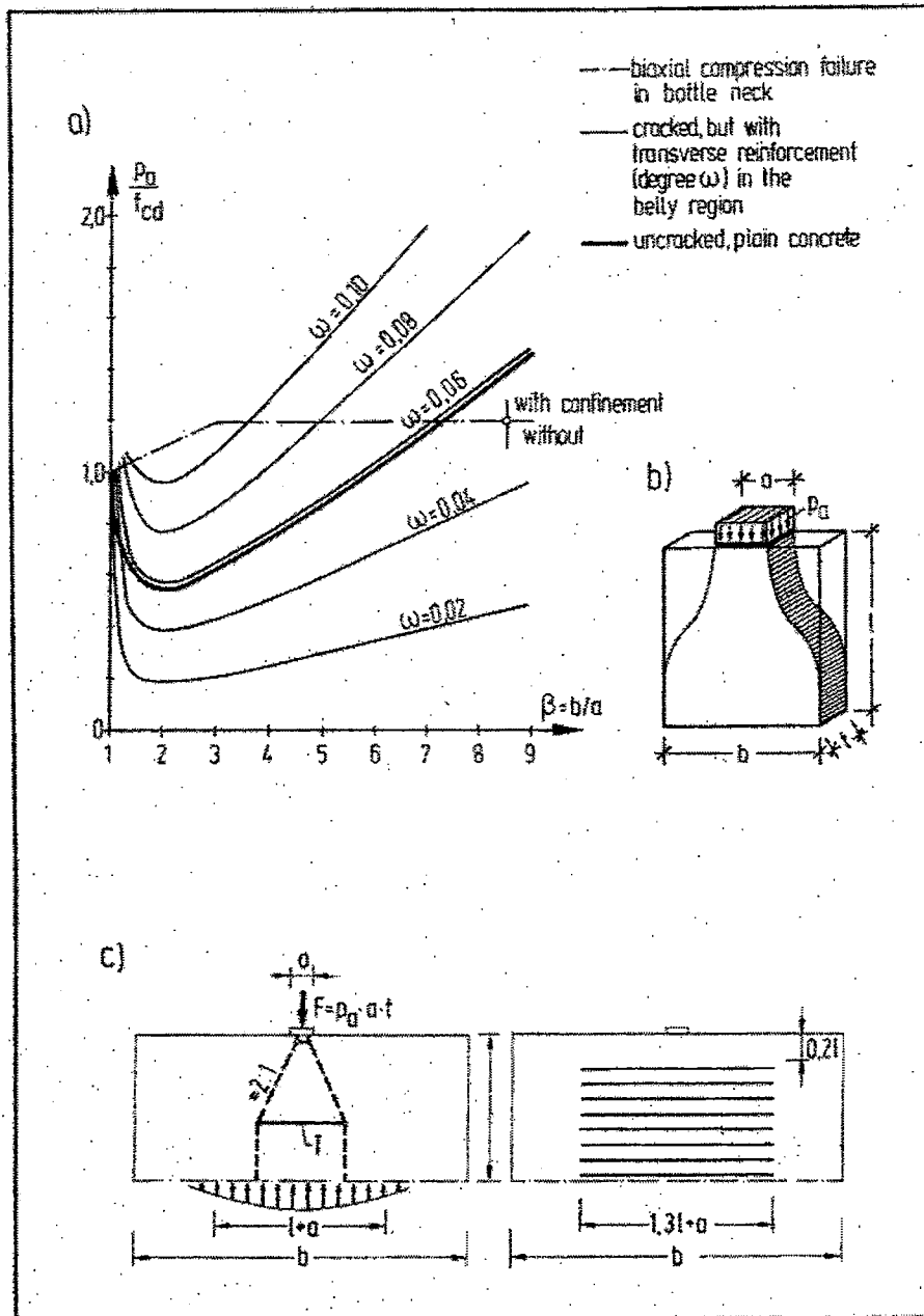
Fig. 23. Dimensioning plane bottle shaped stress fields: (a) diagrams giving safe pressure values P_0 with regard to cracking and crushing of plain unreinforced concrete stress fields, yielding of transverse reinforcement and biaxial compression failure in the bottle neck region; (b) geometry of the stress field; (c) model and reinforcement layout of stress field with transverse reinforcement \omega .
