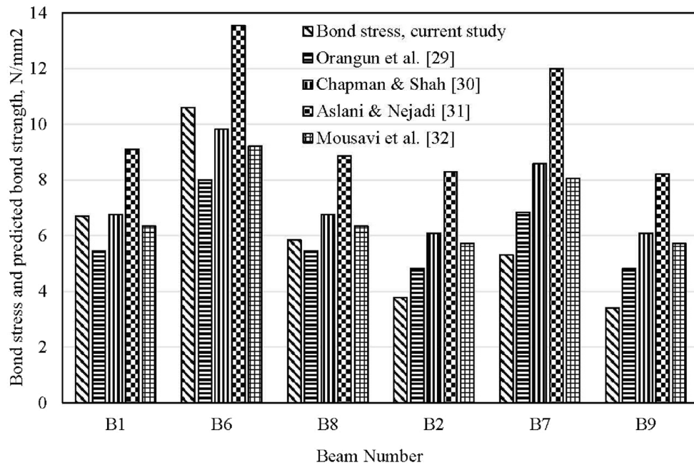
Fig. 23 Bond stress results in the current study and those predicted by other researchers
