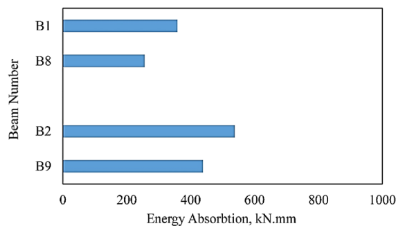
Fig. 19 Energy absorption for beams B1, B2, B8, and B9
