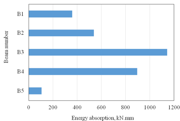
Fig. 7 Energy absorption for Group 1
