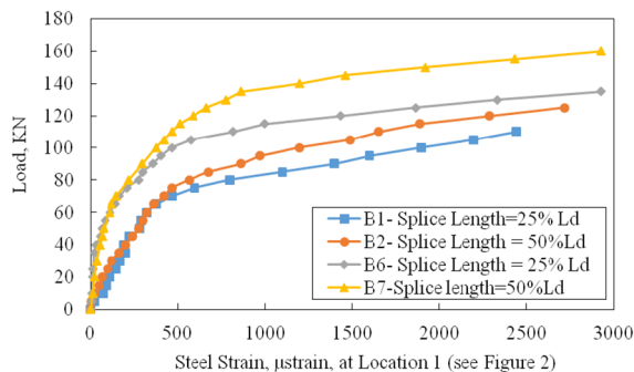
Fig. 17 Load–longitudinal steel strain of Beams B1, B2, B6 and B7
