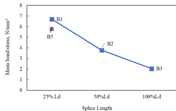
Fig. 8 Bond stress for Beams B1, B2, B3, and B5 (at strain location 1, see Fig. 2)
