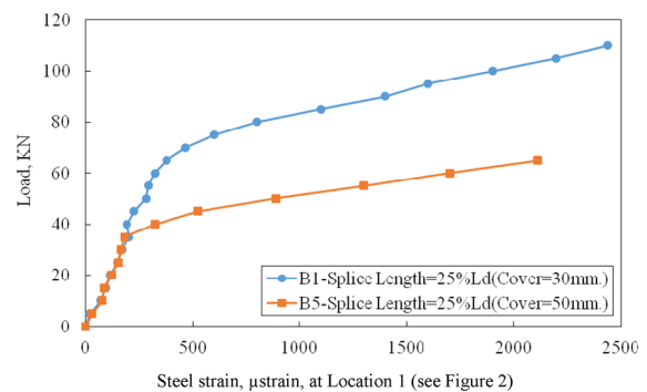
Fig. 12 Load-longitudinal steel strain of Beams B1 and B5
