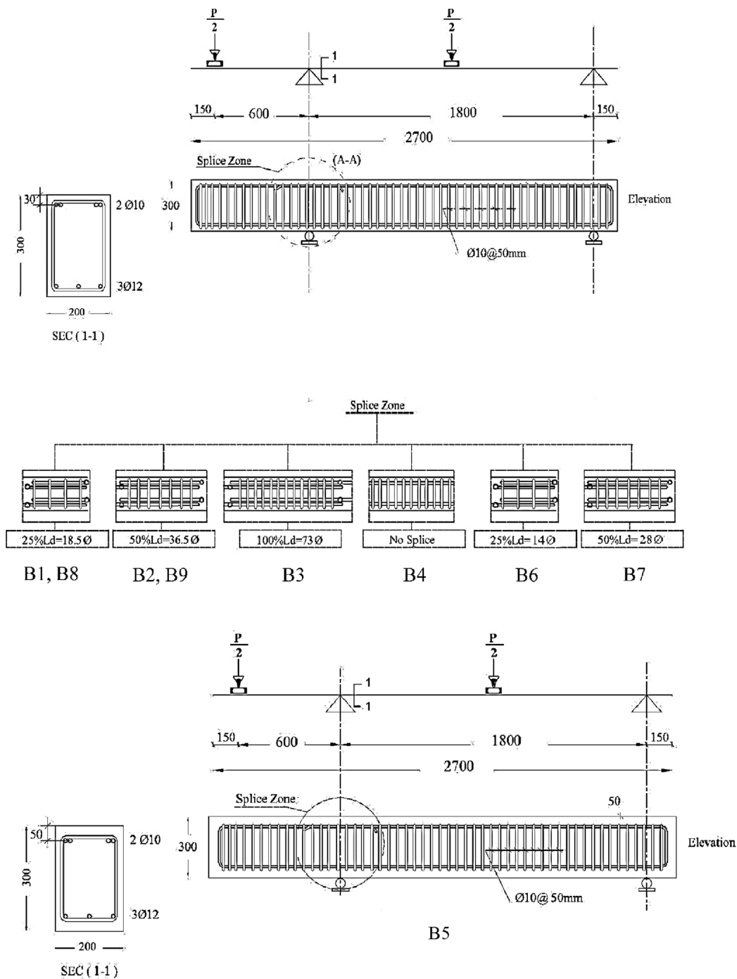
Fig. 3 Geometry and dimensions of studied specimens
