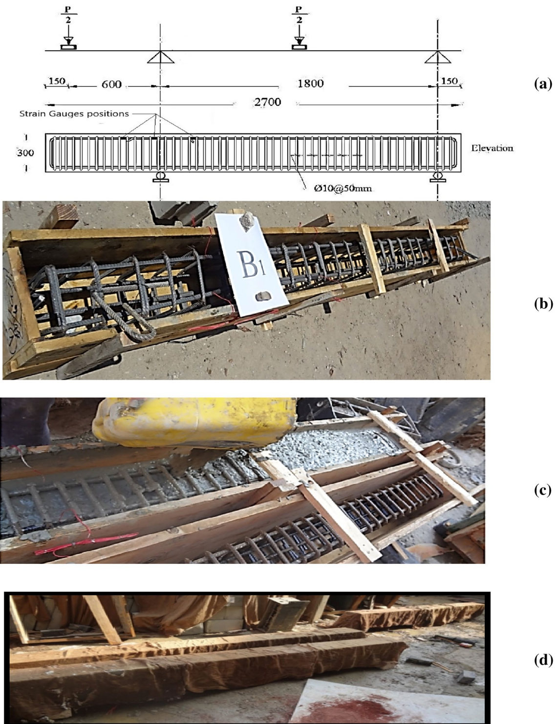
Fig. 2 a Electrical strain gauges' locations, b and reinforcement cage, c casting a typical beam. d Curing of specimens
