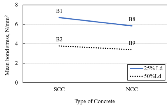
Fig. 20 Bond stress along the lap splice of beams B1, B2, B8 and B9
