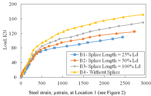
Fig. 10 Load-longitudinal steel strain of Beams B1, B2, B3 and B4
