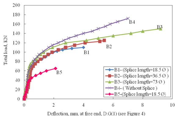
Fig. 6 Load–deflection curves for Group 1 (B1, B2, B3, B4, and B5)
