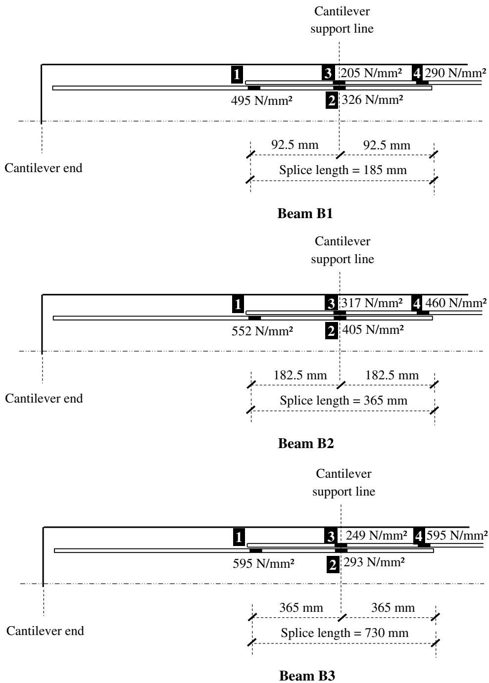
Fig. 9 Ultimate steel stress values calculated from steel strains at strain gauges' locations. Values over 586 N/mm 2 indicate yielding. (Shear links omitted for clarity) Not to scale
