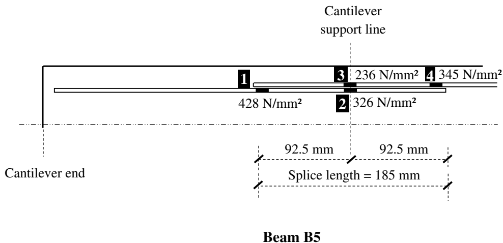
Fig. 11 Ultimate steel stress values calculated from steel strains at strain gauges' locations shown in Fig. 2 (Shear links omitted for clarity) Not to scale
