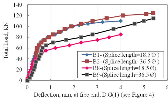
Fig. 18 Load–deflection curves for B1, B2, B8 and B9
