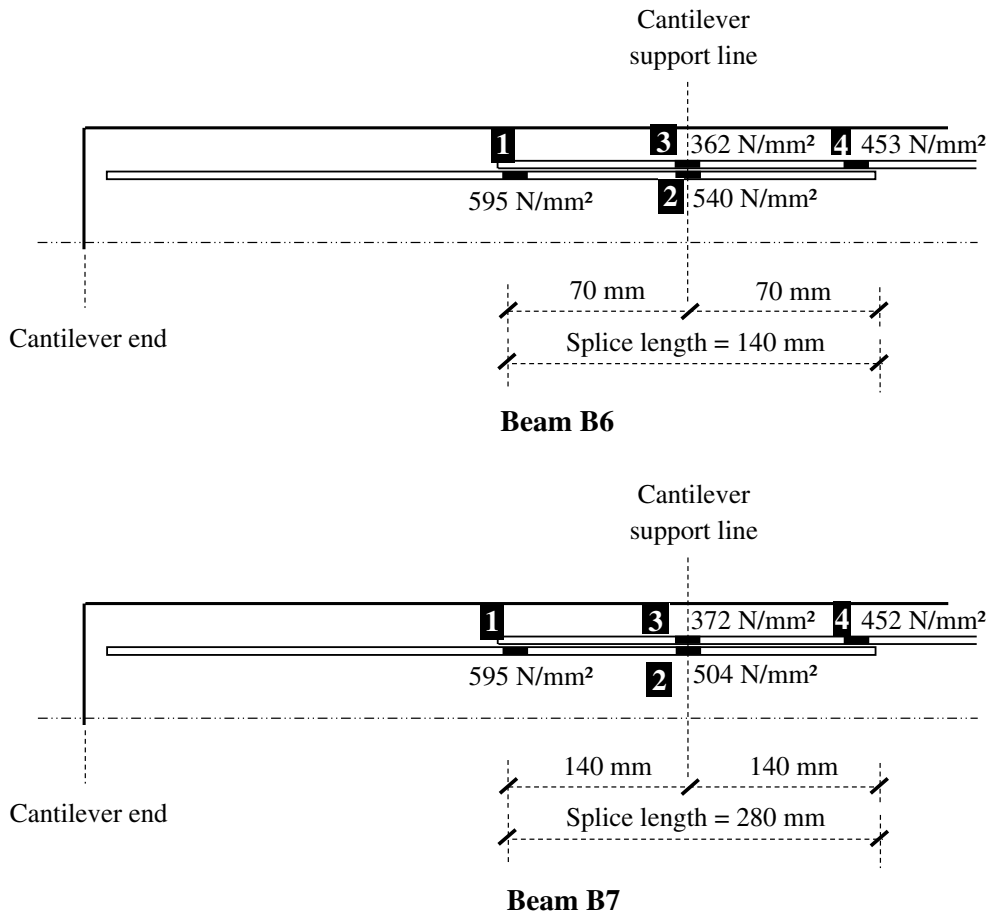
Fig. 16 Ultimate steel stress values calculated from steel strains at strain gauges' locations shown in Fig. 2 (Shear links omitted for clarity) Not to scale
