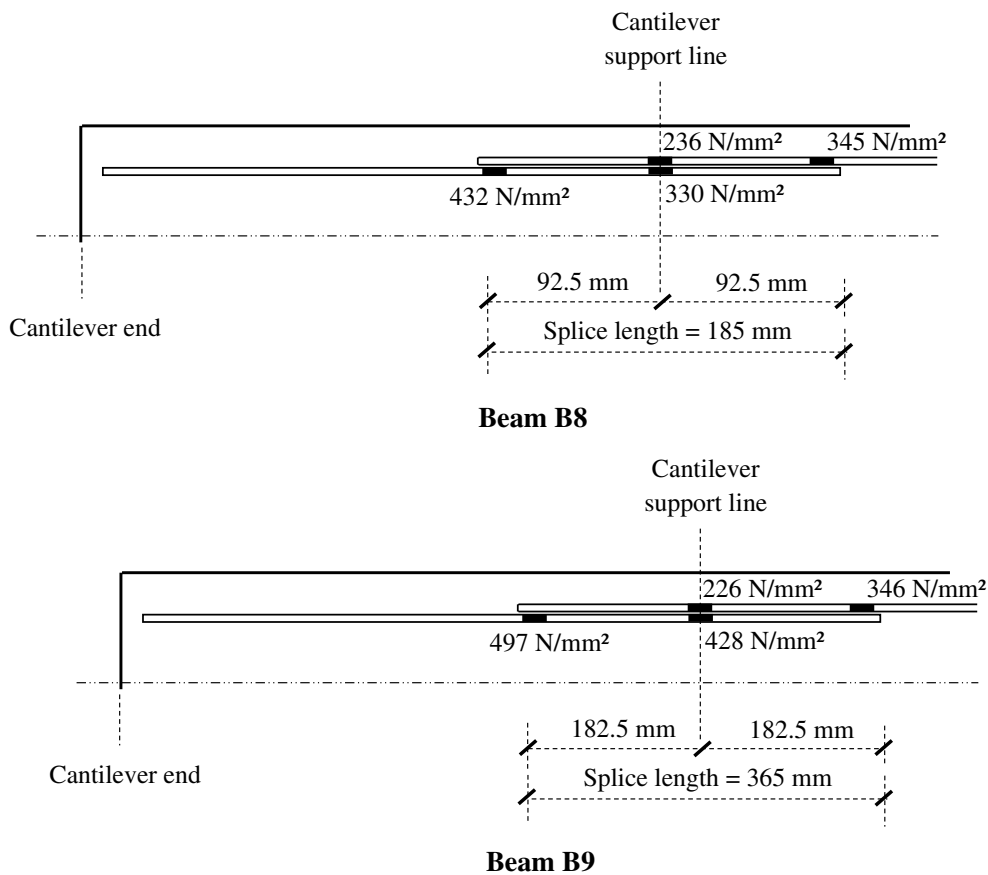
Fig. 21 Ultimate steel stress values calculated from steel strains at strain gauges' locations shown in Fig. 2 (Shear links omitted for clarity) Not to scale
