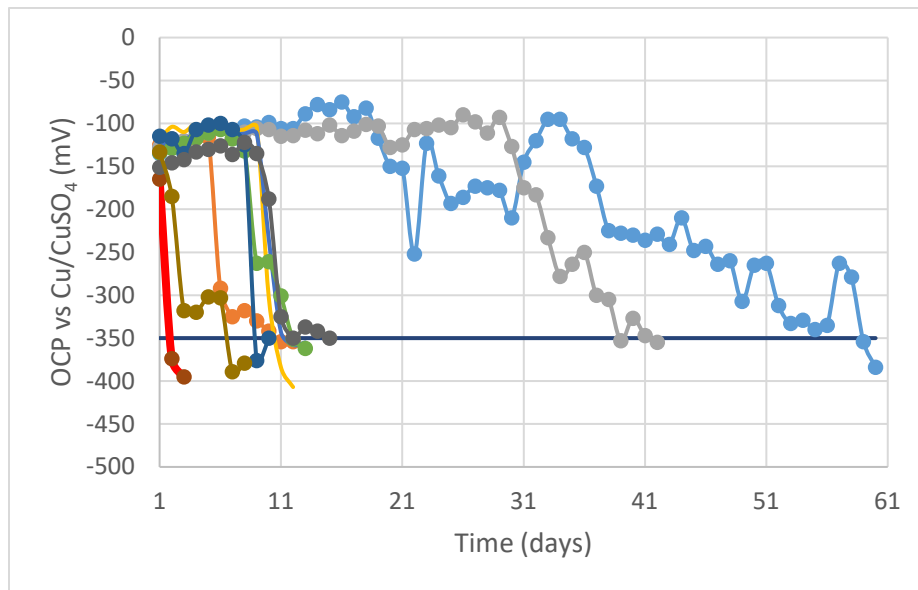
Figure 22 OCP vs Cu/CuSO 4 for S1 in C1 at WJE
