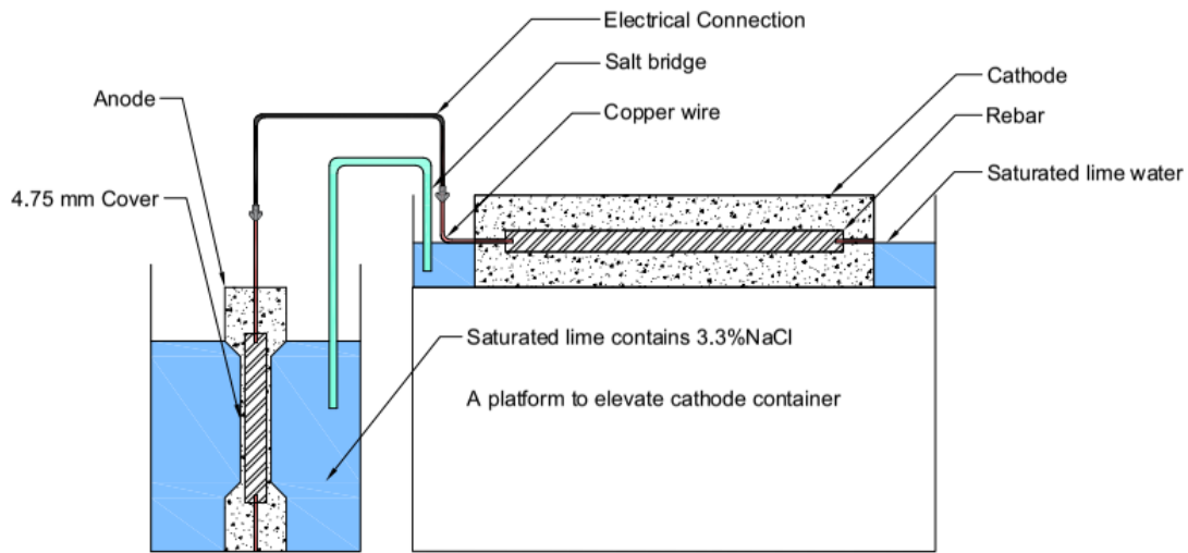
Figure 1 OC_{crit} Test Setup
