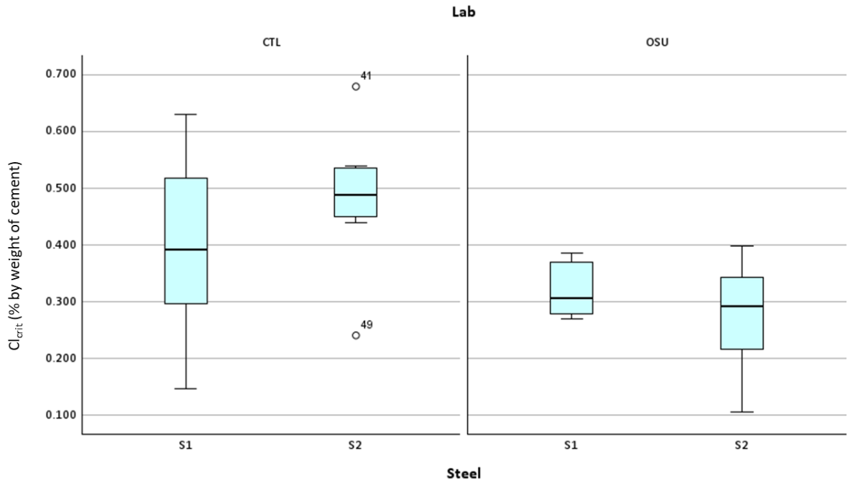
Figure 20 Cl_{crit} distributions for Steel Samples S1 and S2 measured at CTLGroup and OSU labs.
