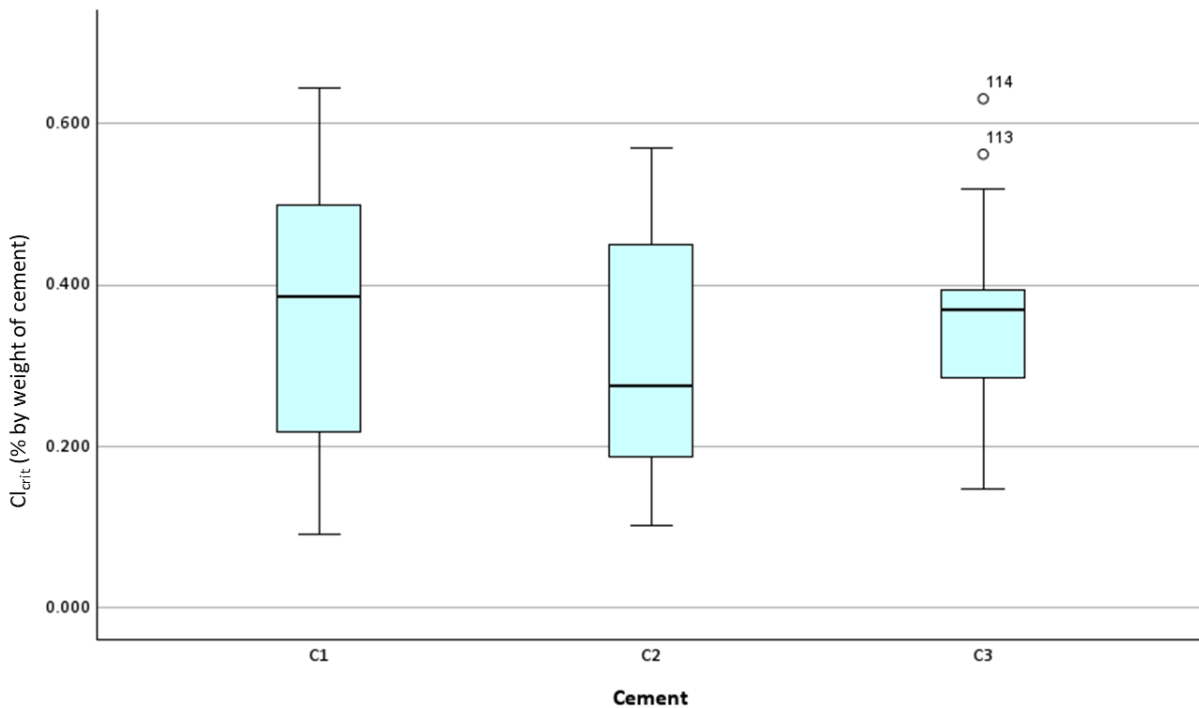
Figure 26 Cl_{crit} distributions for S1 samples in mortar made with C1, C2, and C3
