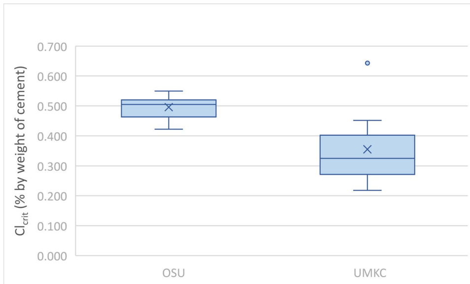
Figure 9 Cl_{crit} distributions for S1 samples in C1 at UMKC and OSU
