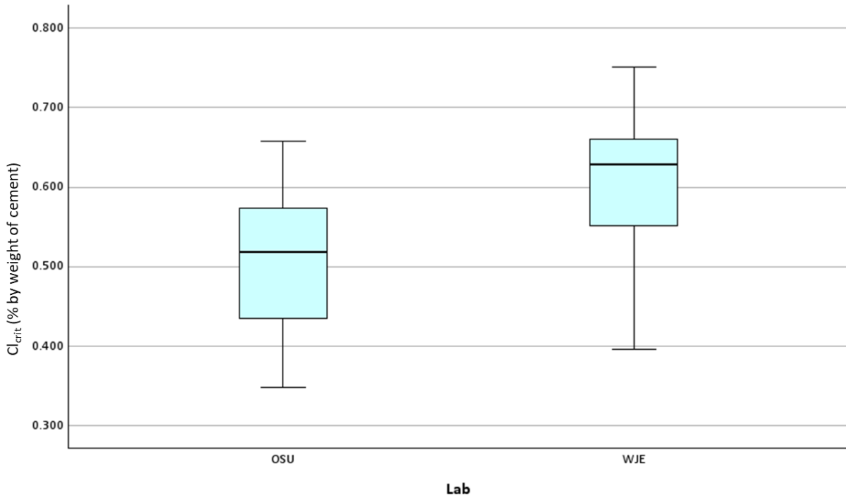
Figure 25 Cl_{crit} distributions for S3 samples in C1 cement measured at OSU and WJE labs
