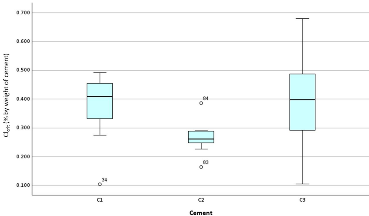
Figure 30 Cl_{crit} distributions for S2 samples in mortar made with C1, C2, and C3
