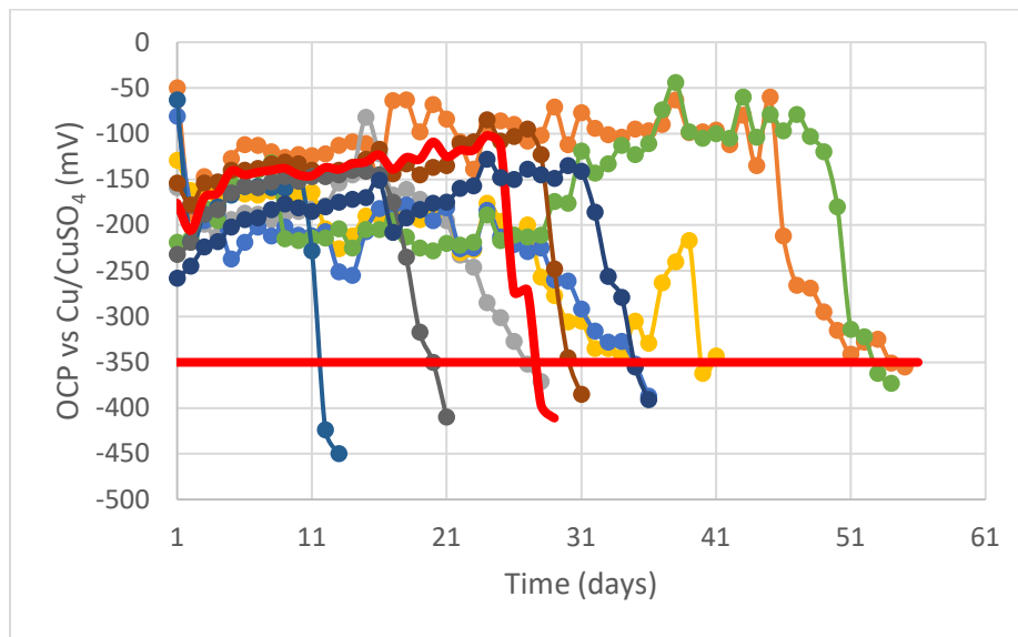
Figure 4 OCP vs Cu/CuSO 4 for S1 in C1 at UMKC
