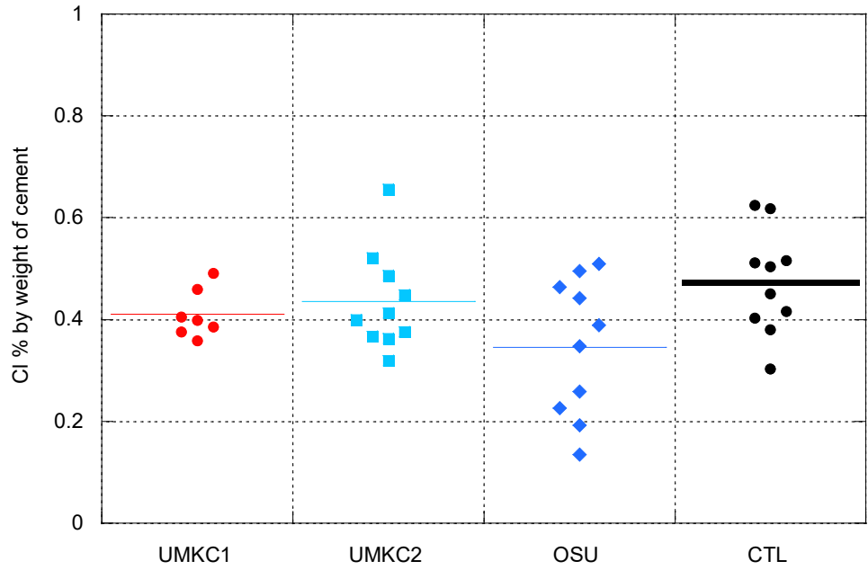
Figure 2 OC_{crit} First Phase Study Cl_{crit} Distributions
