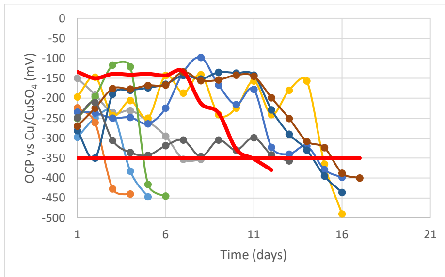
Figure 5 OCP vs Cu/CuSO_4 for S1 in C2 at UMKC
