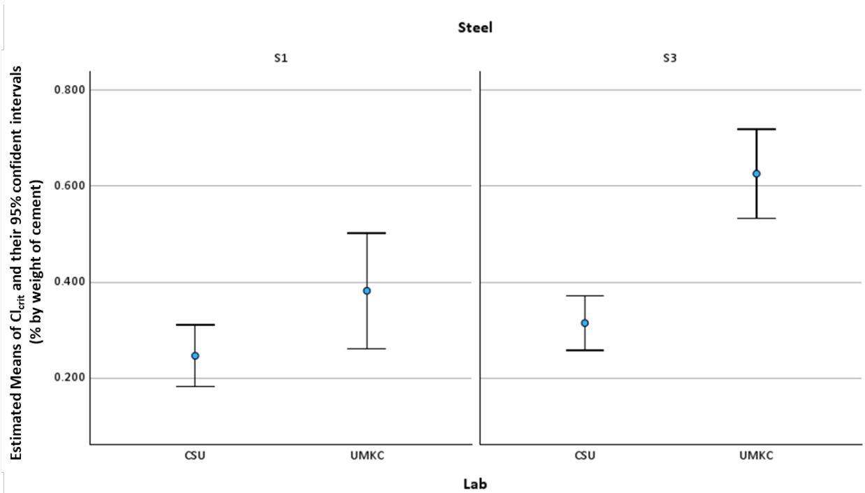
Figure 16 Cl_{crit} distributions for Steel Samples S1 and S3 measured at CSU and UMKC labs.
