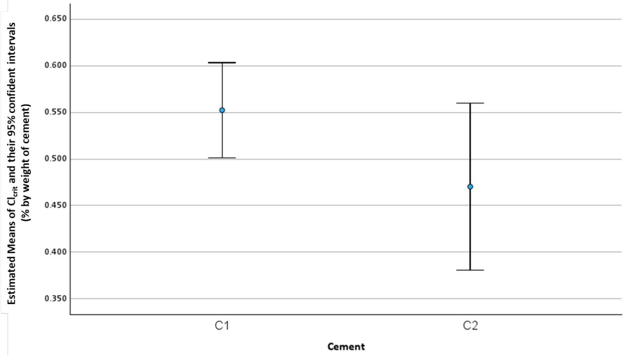
Figure 35 Mean Cl_{crit} values and 95% confidence intervals for S3 steel in C1 and C2 cement mortar
