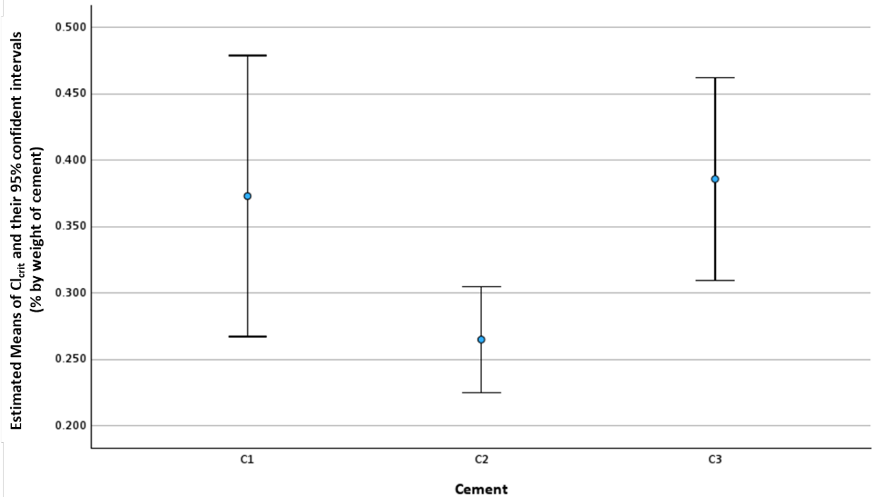
Figure 31 Mean Cl_{crit} values and 95% confidence intervals for S2 steel in C1, C2, and C3 cement mortar
