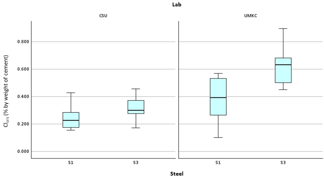
Figure 16 Cl_{crit} distributions for Steel Samples S1 and S3 measured at CSU and UMKC labs.
