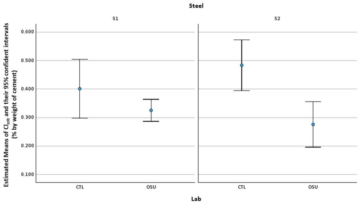
Figure 21 Mean Cl_{crit} values and 95% confidence intervals at CTLGroup and OSU for Steel S1 and S2
