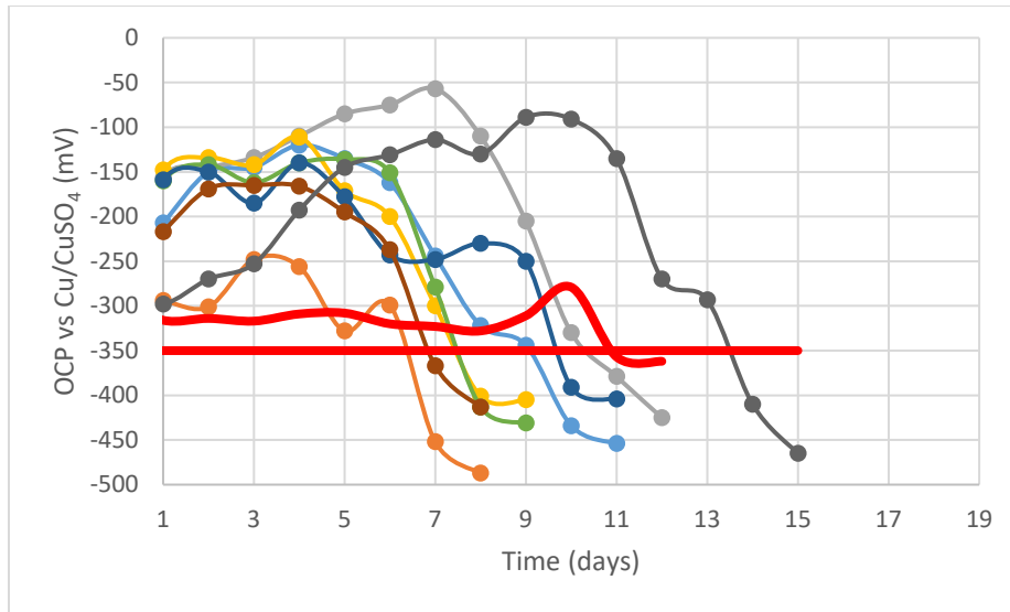
Figure 11 OCP vs Cu/CuSO 4 for S1 in C3 at OSU
