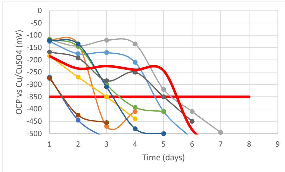
Figure 15 OCP vs Cu/CuSO 4 for S3 in C2 at CSU
