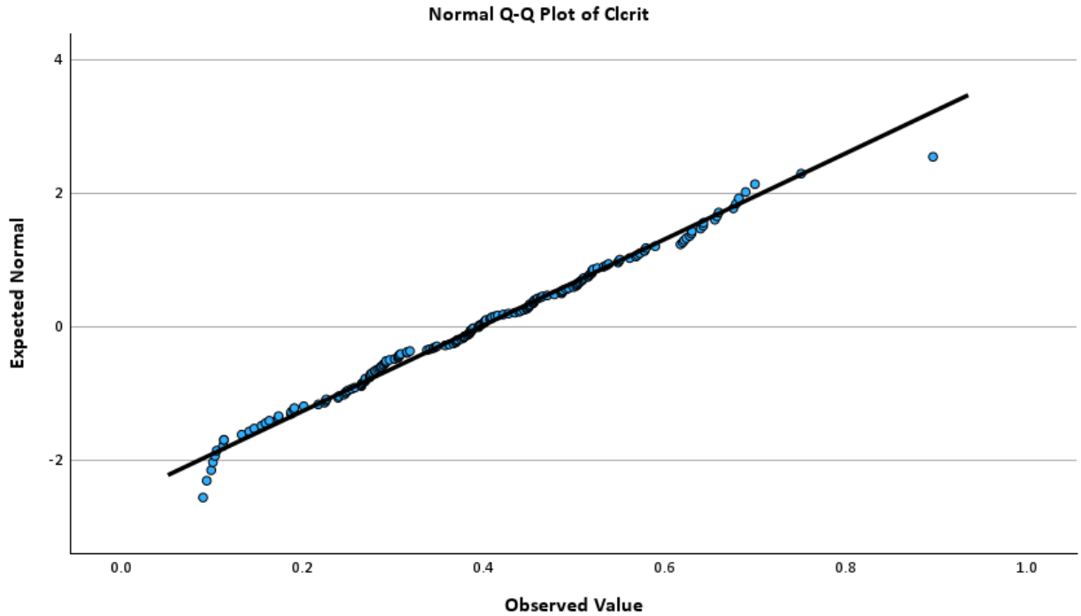
Figure 43 QQ Plot for the combined Cl_{crit} data of Phases I and II
