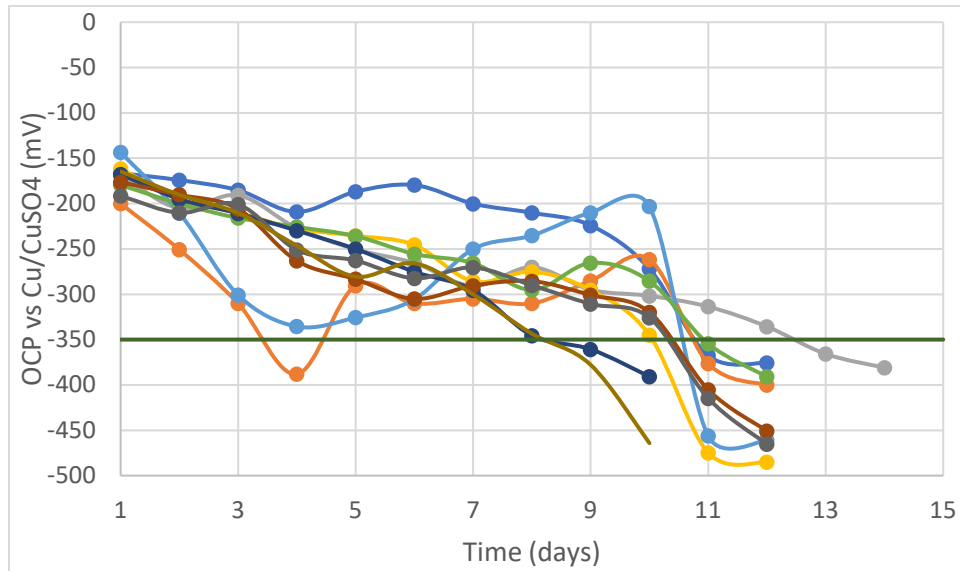
Figure 7 OCP vs Cu/CuSO 4 for S3 in C2 at UMKC
