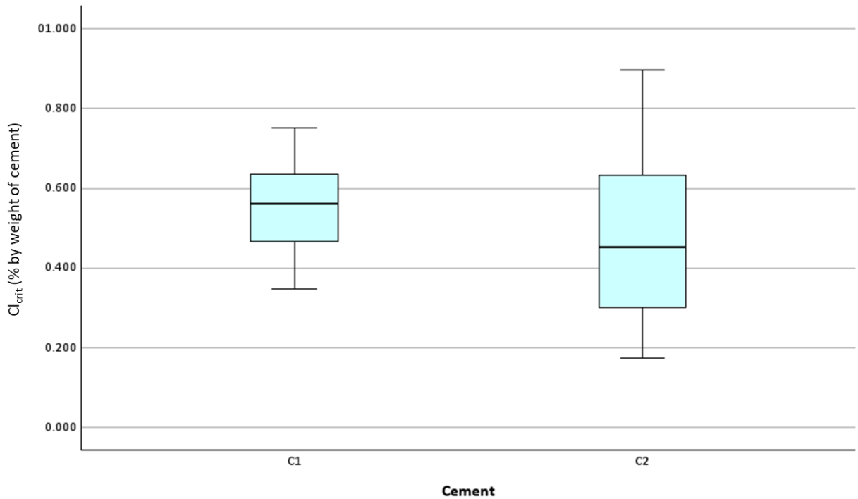
Figure 34 Cl_{crit} distributions for S3 samples in mortar made with C1 and C2
