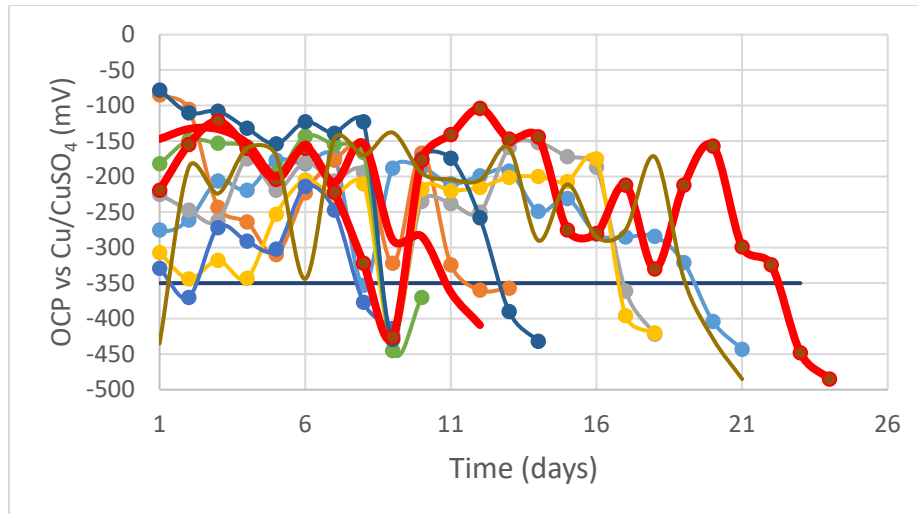
Figure 10 OCP vs Cu/CuSO 4 for S3 in C1 at OSU
