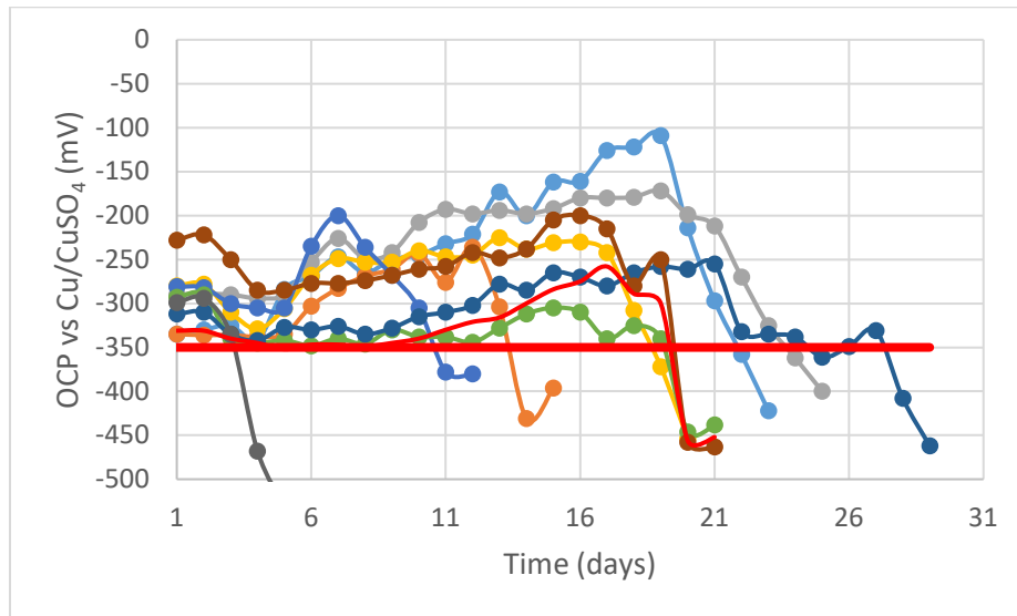
Figure 18 OCP vs Cu/CuSO 4 for S1 in C3 at CTLGroup
