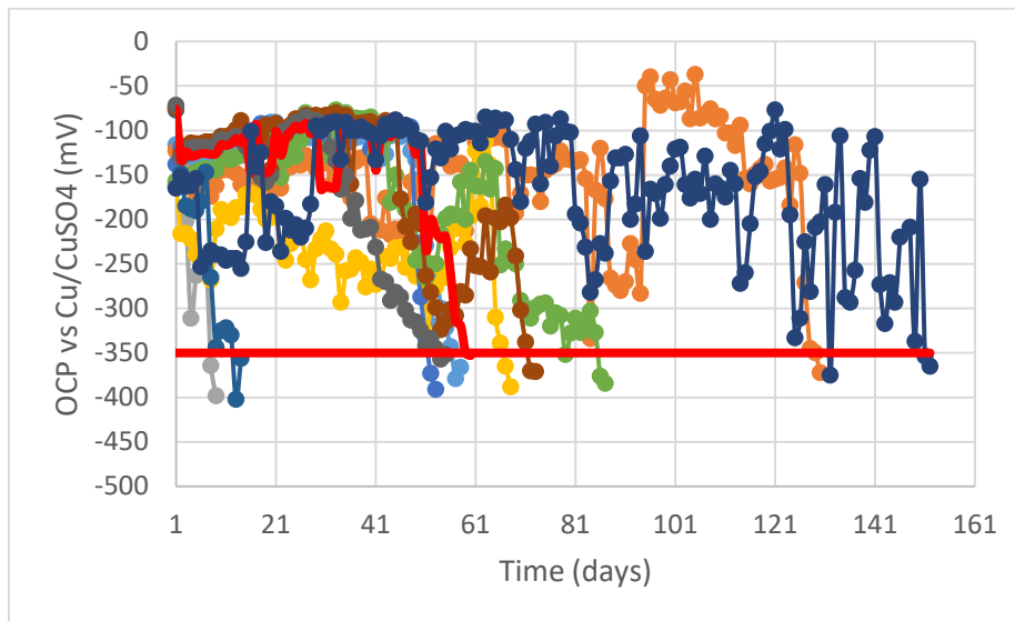
Figure 6 OCP vs Cu/CuSO_4 for S2 in C1 at UMKC
