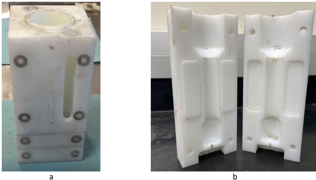
Figure 3 OC_{crit} Mold Designs in First and Second Phase Studies
