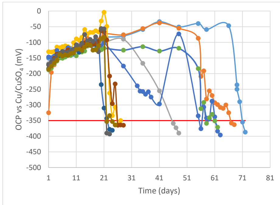
Figure 24 OCP vs Cu/CuSO 4 for S3 in C1 at WJE
