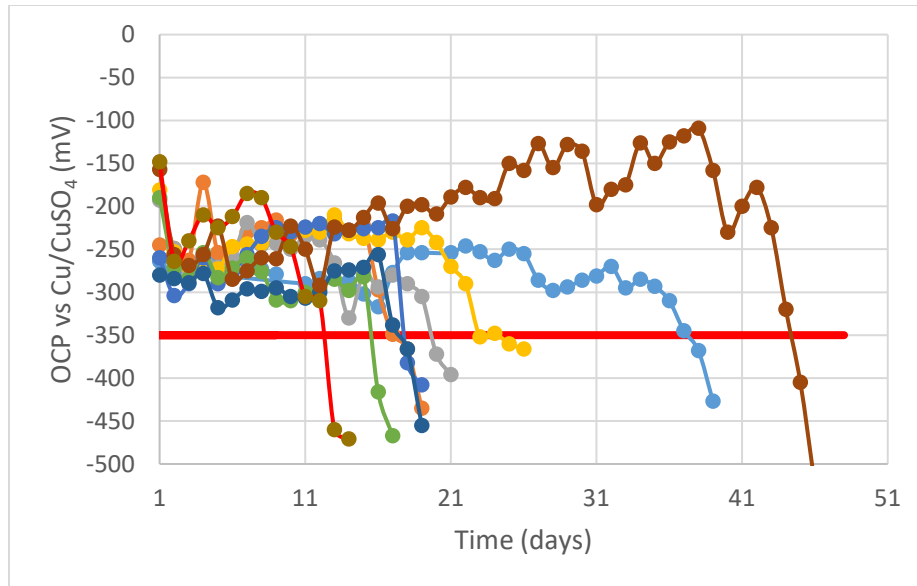
Figure 19 OCP vs Cu/CuSO 4 for S2 in C3 at CTLGroup
