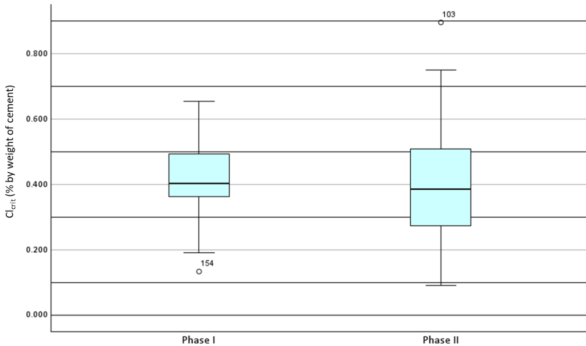
Figure 40 Cl_{crit} distributions for all samples in Phases I and II
