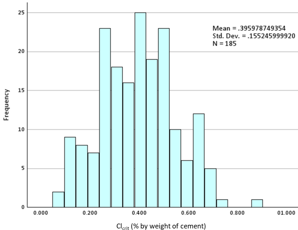
Figure 42 Histogram of the combined Cl crit data of Phases I and II
