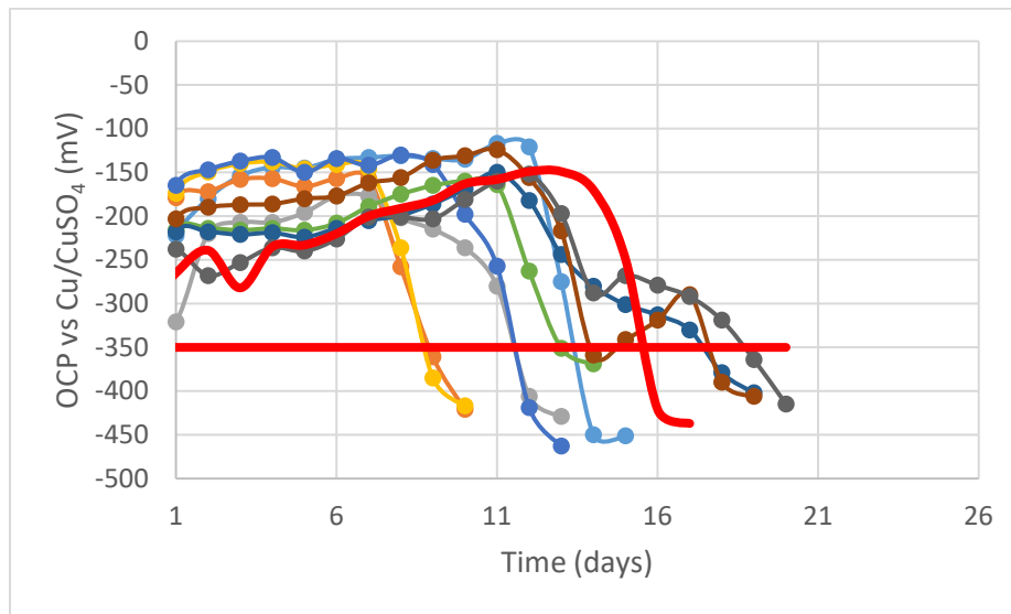
Figure 8 OCP vs Cu/CuSO 4 for S1 in C1 at OSU
