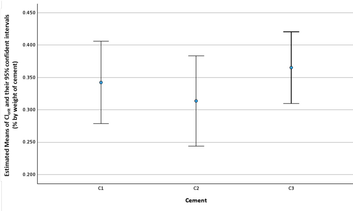
Figure 27 Mean Cl_{crit} values and 95% confidence intervals for S1 steel in C1, C2, and C3 cement mortar
