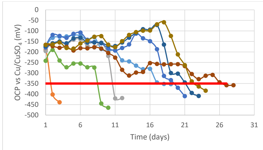
Figure 12 OCP vs Cu/CuSO 4 for S2 in C3 at OSU
