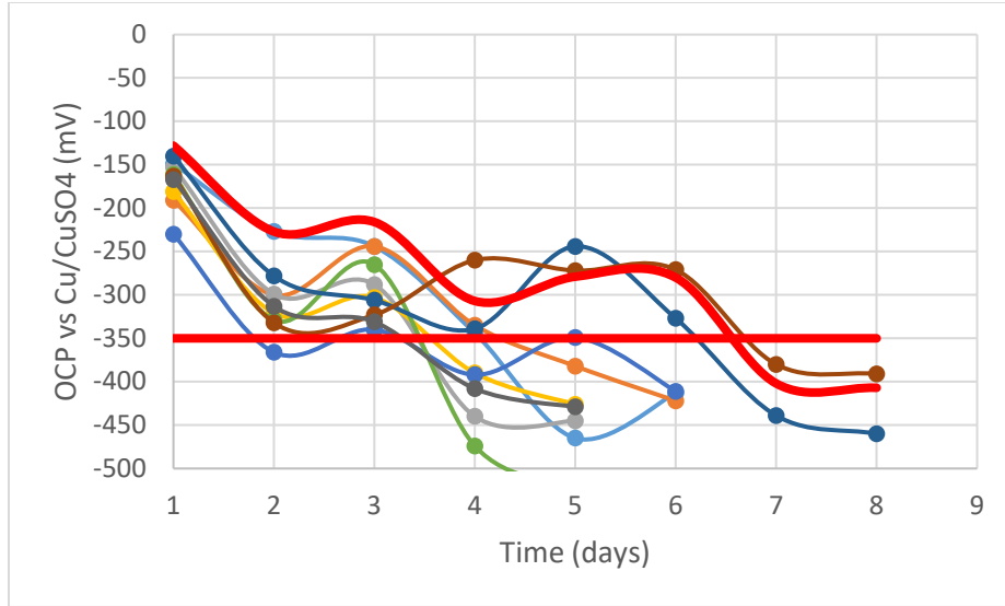
Figure 14 OCP vs Cu/CuSO 4 for S2 in C2 at CSU
