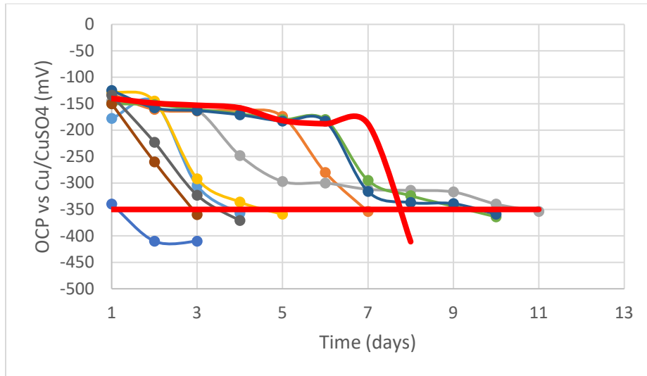
Figure 13 OCP vs Cu/CuSO 4 for S1 in C2 at CSU
