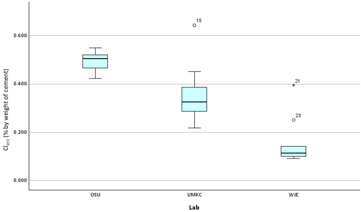
Figure 23 Cl_{crit} distributions for S1 samples in C1 cement measured at OSU, UMKC, and WJE labs.
