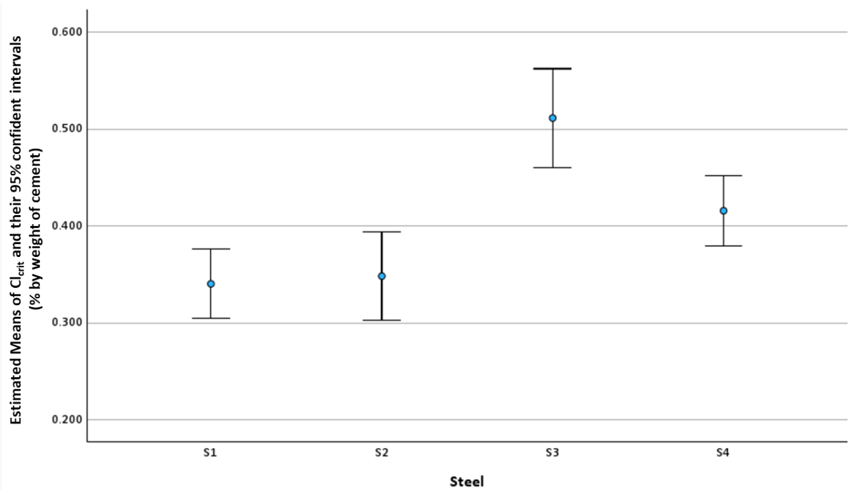
Figure 37 Cl_{crit} distributions for all samples separated by steel source including the first phase study
