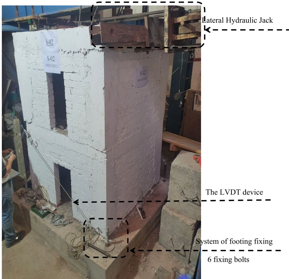
Fig. 6 Test configuration
