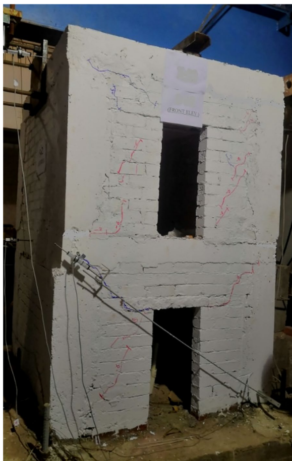
Fig. 9 The first obvious cracks S-01 (front)
