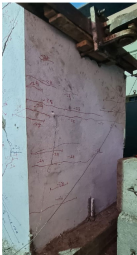
Fig. 20 Failure crack pattern S-02 (right)
