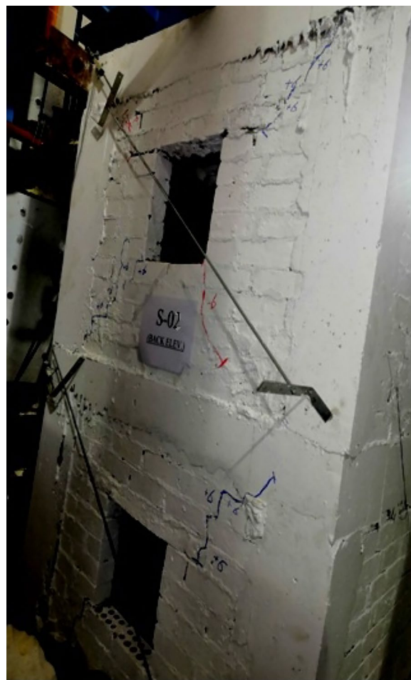
Fig. 10 The first obvious cracks S-01 (back)
