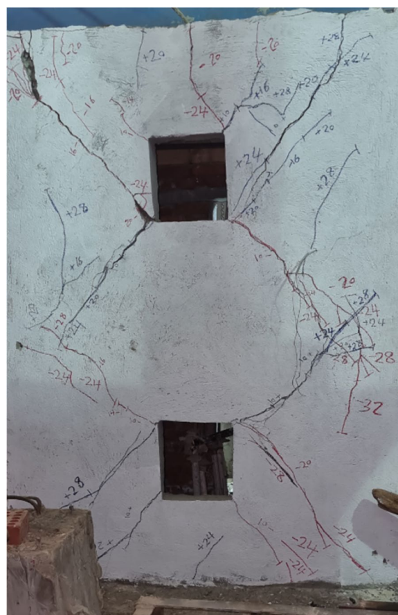
Fig. 18 Failure crack pattern S-02 (back)
