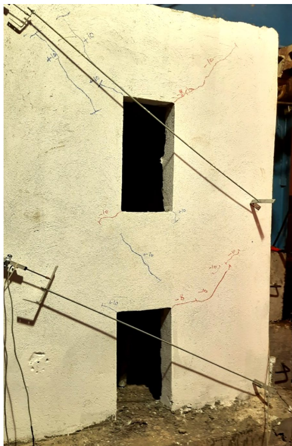
Fig. 15 The first obvious cracks S-02 (front)
