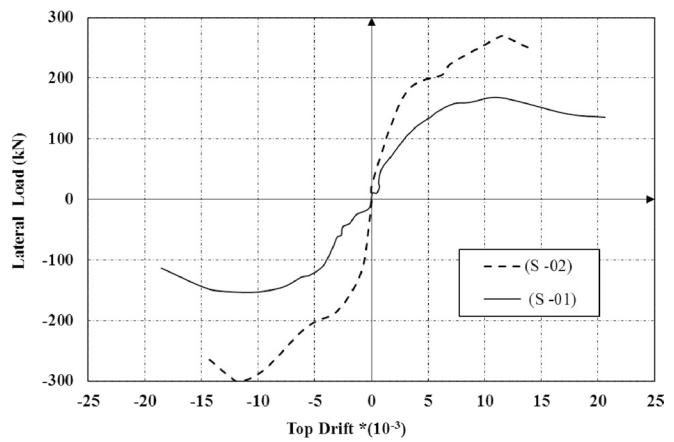
Fig. 21 Strengthened and un-strengthened assemblies' hysteretic curves. a Un-strengthened 3D assembly (S-01) ((Displacement and drift) b Strengthened 3D assembly (S-02) (Displacement and drift)
