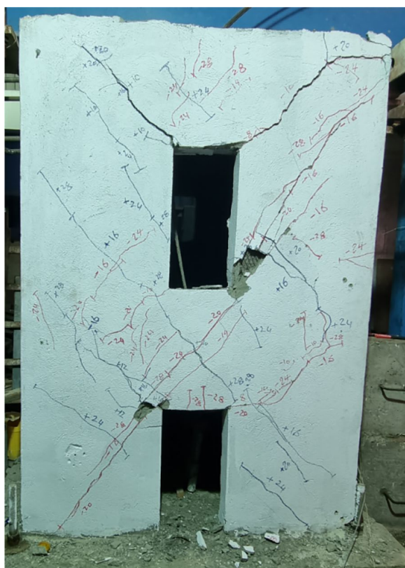
Fig. 17 Failure crack pattern S-02 (front)
