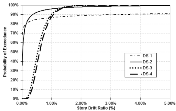
Fig. 38 Drift fragility curve for the building
